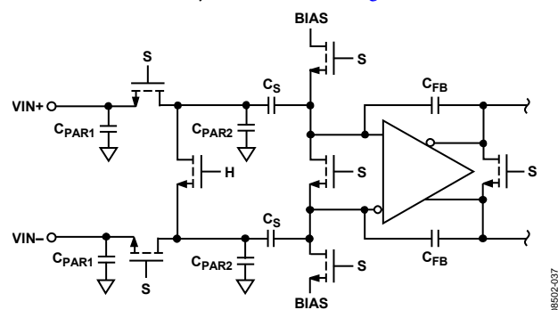
Figure 64. Switched Capacitor Input
