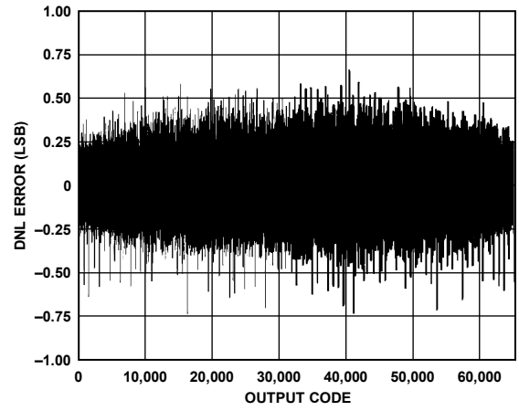
Figure 51. AD9265-125 DNL with f_{IN} = 9.7 MHz
