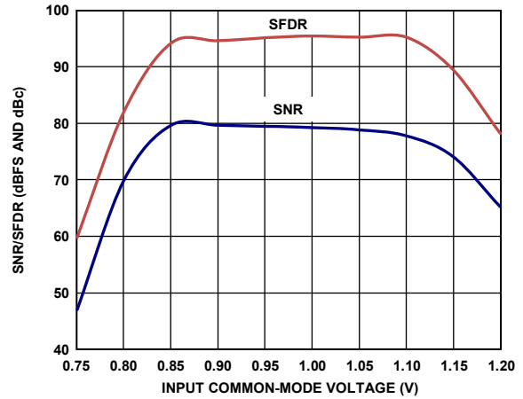
Figure 52. AD9265-125 SNR/SFDR vs. Input Common Mode (VCM) with f_{IN} = 30 MHz
