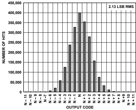
Figure 49. AD9265-125 Grounded Input Histogram
