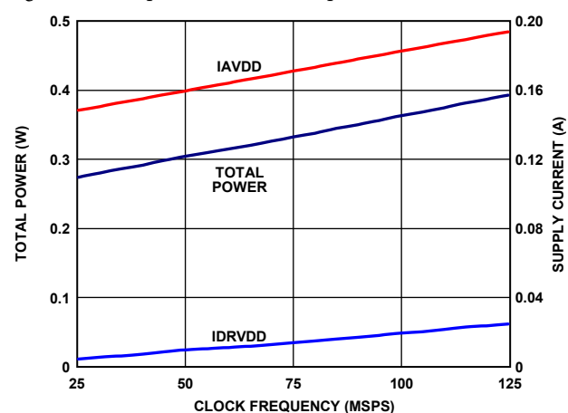
Figure 81. AD9265-125 Power and Current vs. Sample Rate
