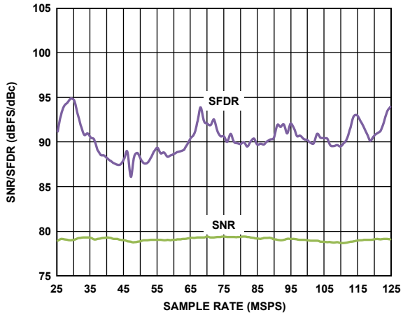
Figure 48. AD9265-125 Single-Tone SNR/SFDR vs. Sample Rate ( f_s ) with f_{IN} = 70.1 MHz
